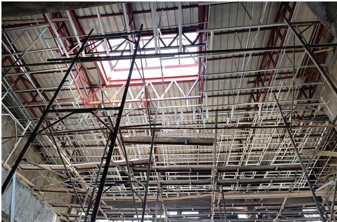
Phase 2 works showing: Brandering for gypsum ceiling at the penthouse
