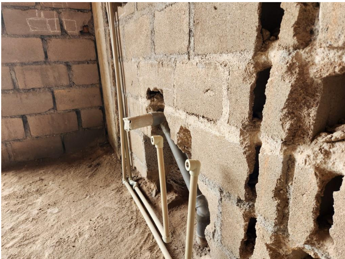
Plumbing works in the kitchen area
